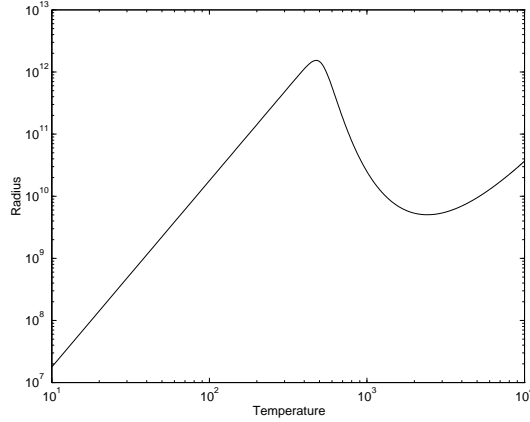
Figure 3: Maximal radius of information processing system as a function of working temperature (as per equation 18, with \rho = 10^{18} bits/m 3 , E = 10^{-19} J and \epsilon = 10^{-6} ).
